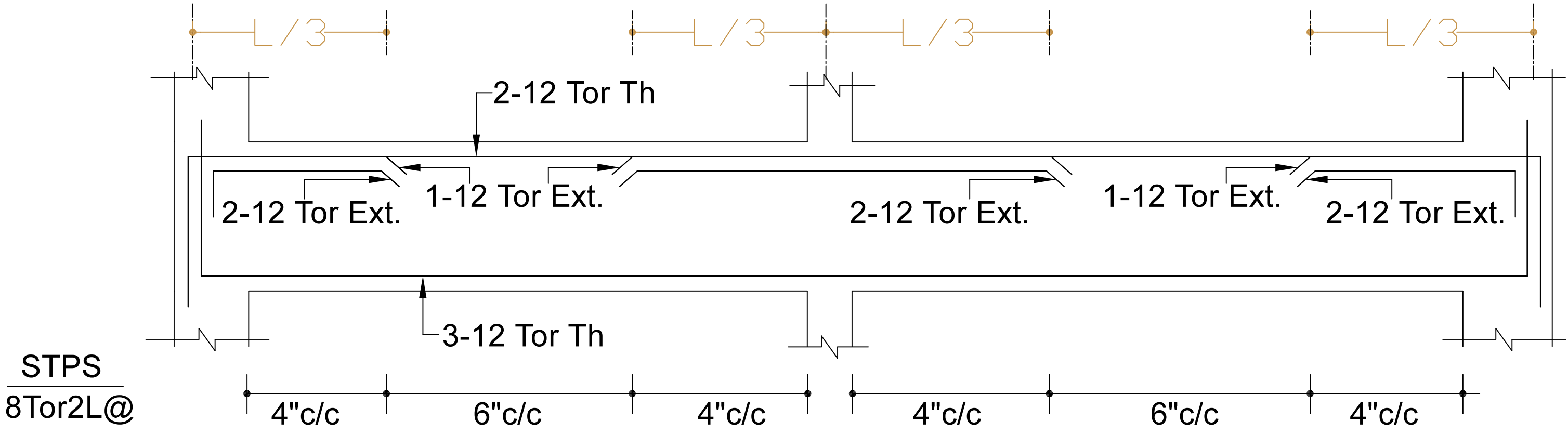
DET. OF TYPICAL TIE BEAM 10"X12"
